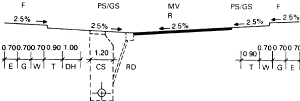
⑧ Basic widths for the supply and drainage pipework layout in the road space
